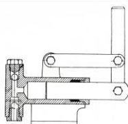
Tender handpomp
